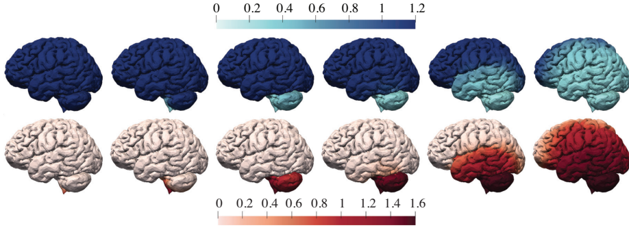
Figure 4. Test case from Section 5. Snapshot of the computed solution c_h(\mathbf{x}, t) (blue) and q_h(\mathbf{x}, t) (red) for t \in \{0, 5, 10, 15, 20, 25\} years.
