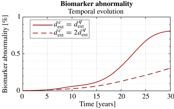
Figure 12. Test case of Section 5.2. Sensitivity analysis for two different mechanisms of extra-cellular diffusion.
