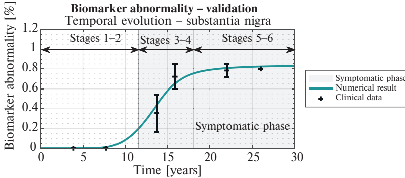
Figure 11. Test case of Section 5.1. Validation for the biomarker abnormality in the substantia nigra brain region. The green line represents the biomarker abnormality curve computed from the numerical results obtained from the simulation of Section 5. Clinical data are taken from [8, Table 2]. The severity of the disease is mapped on the range [0, 0.8] , and for each stage, we take the average value and show the symmetric interval with amplitude twice the standard deviation.
