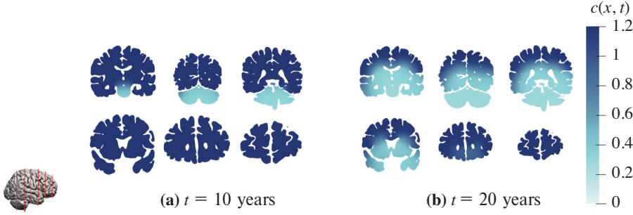
Figure 9. Test case from Section 5. Evaluation of healthy protein loss at 10 and 20 years, observed across six coronal sections within the three-dimensional domain shown on the left.
