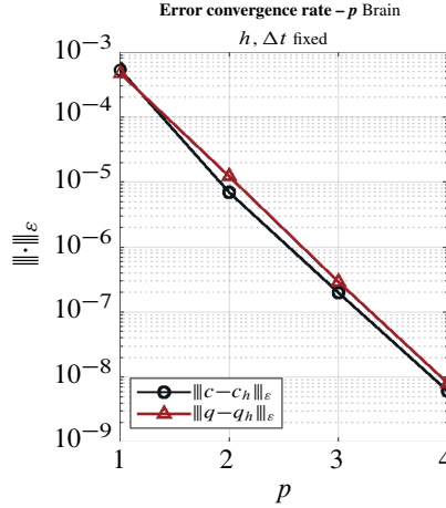
Figure 3. Test case of Section 4.1.2. Computed errors in the \| \cdot \|_\varepsilon norm versus the polynomial degree of approximation (semilog scale) for \Delta t = 5 \cdot 10^{-6} .
