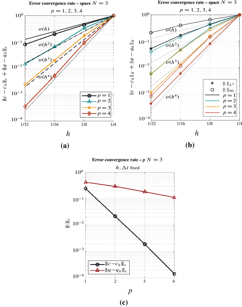
Figure 1. Test case of Section 4.1.1. (a) Computed errors in the \|\cdot\|_\varepsilon norm versus the mesh size h (loglog scale) for different polynomial approximation degrees p = 1, 2, 3, 4 . (b) Computed errors in the \|\cdot\|_{L^2(\Omega)} and \|\cdot\|_{DG} norms versus the mesh size h (loglog scale) for different polynomial approximation degrees p = 1, 2, 3, 4 . (c) Computed errors in the \|\cdot\|_\varepsilon norm versus the polynomial degree of approximation (semilog scale) for h = 1/4 , \Delta t = 5 \cdot 10^{-6} .
