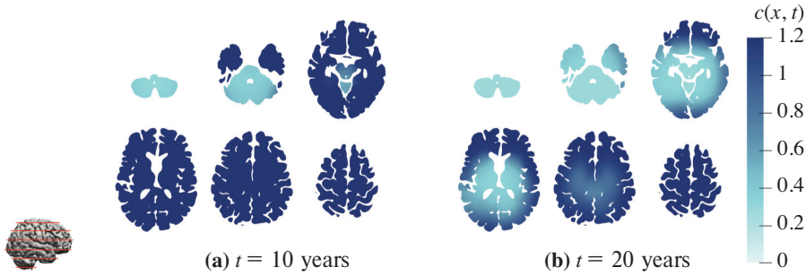
Figure 7. Test case from Section 5. Evaluation of healthy protein loss at 10 and 20 years, observed across six transversal sections within the three-dimensional domain shown on the left.
