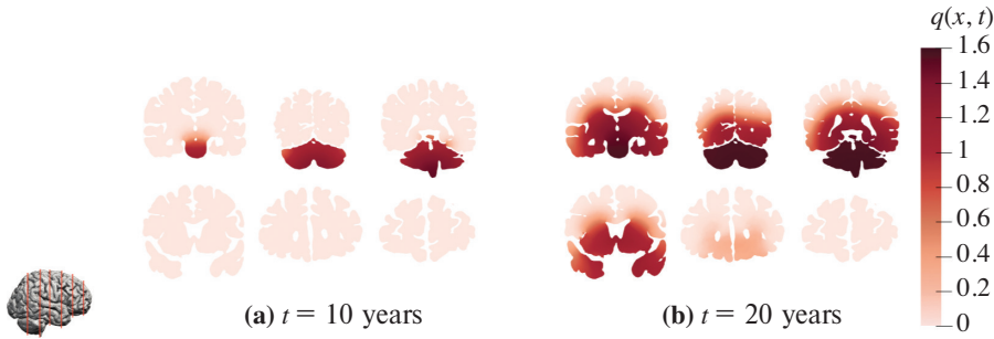
Figure 10. Test case from Section 5. Evaluation of misfolded protein diffusion at 10 and 20 years, observed across six coronal sections within the three-dimensional domain shown on the left.
