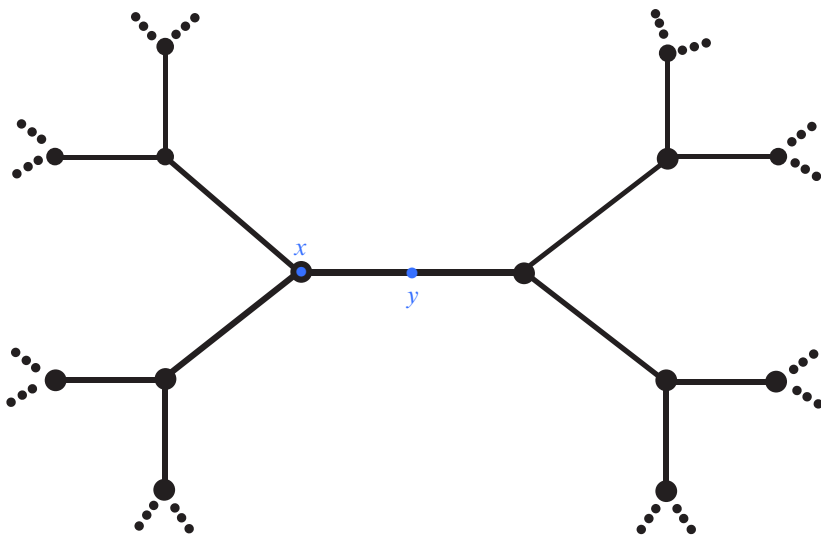
Figure 2. Bruhat–Tits building for G = \mathrm{SL}_2(\mathbb{Q}_2) .
