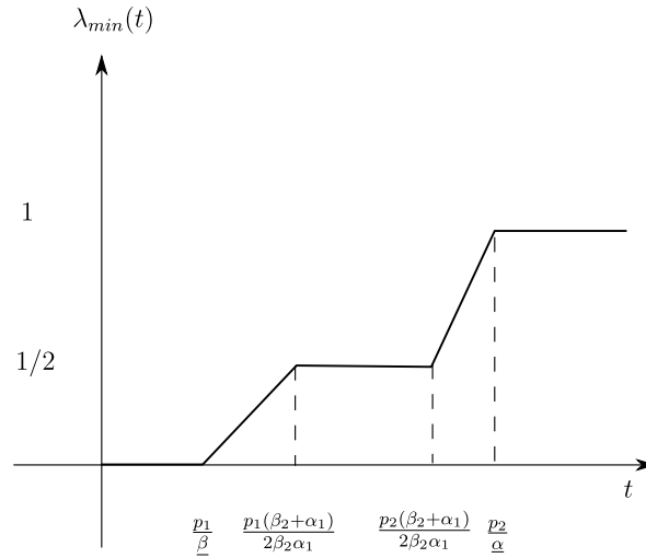
Fig. 2. The value of \lambda_{\min} .
