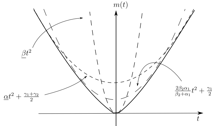
Fig. 1. The minimal value m .
