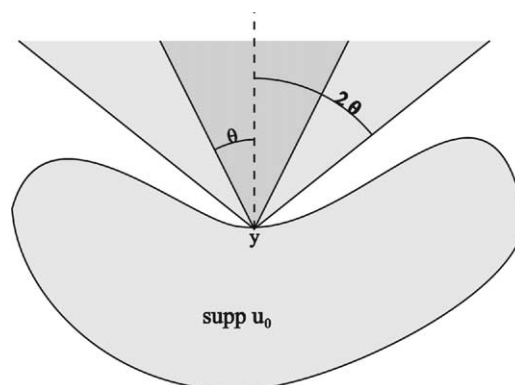
Fig. 1. Provided initial data are sufficiently smooth in a neighborhood of y , the solution u stays zero for finite time within the inner cone.
