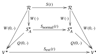
Fig. 1. Commutative diagram.
