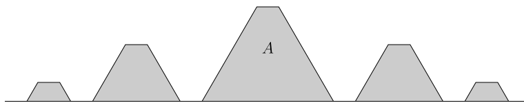
Fig. 7. The closed set A , whose boundary contains L and S(L) (with N = 37 ).
