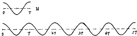
FIG. 2. Functions in M defined by (3.10) for the case of k=5 , where u \in SE_T^- .
