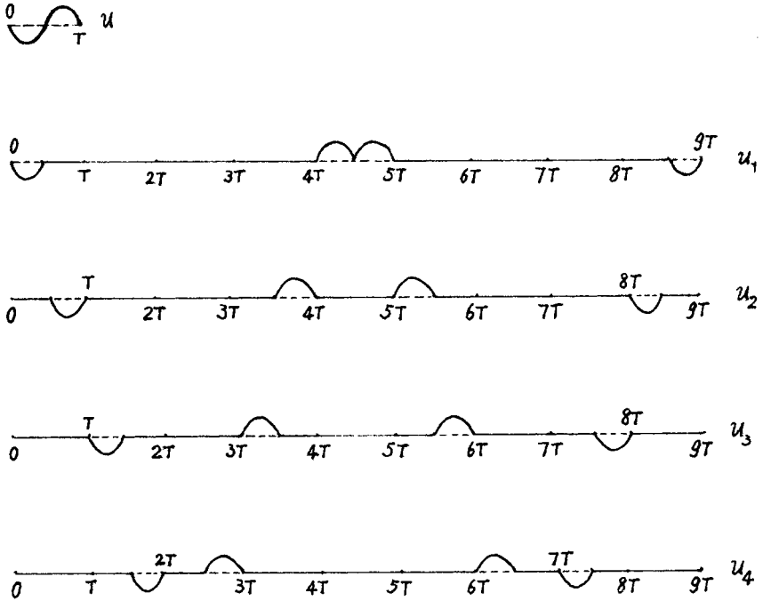
FIG. 1. Functions in N_i defined by (3.8) for the case of k=9 , where u \in AE_T^0 .
