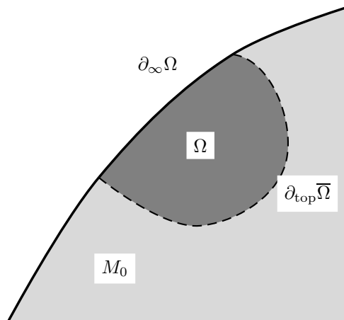
FIGURE 1. A regular open set \Omega . Note that the interior of \partial_{\infty}\bar{\Omega} is contained in \Omega , but the true boundary \partial_{\text{top}}\Omega = \partial_{\text{top}}\bar{\Omega} is not contained in \Omega
