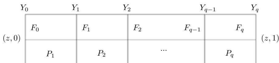
Figure 3: Sequence of walls meeting the geodesic
