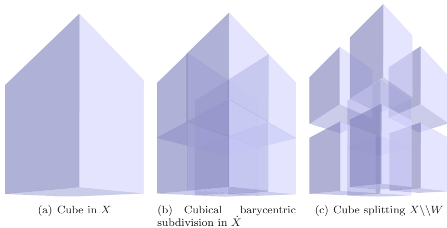
Figure 1: Subdividing and splitting a cube complex
