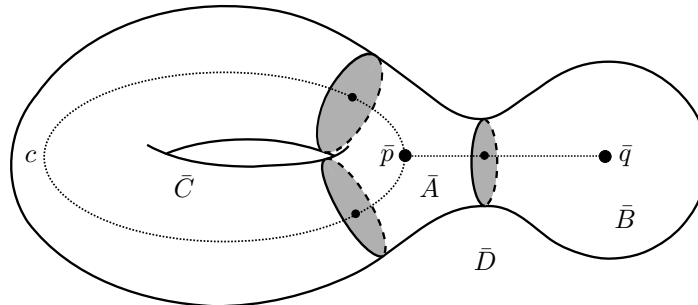
Figure 7: Decomposition of \bar{X}^3 \cong S^3 into four closed sets, where \bar{D} is the complement of the solid torus, \bar{A} \cup \bar{B} \cup \bar{C} , viewed in S^3 \setminus \{\infty\} .
