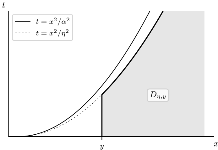
Figure 5. Sketch of the region D_{\eta,y} when \eta > \alpha .
