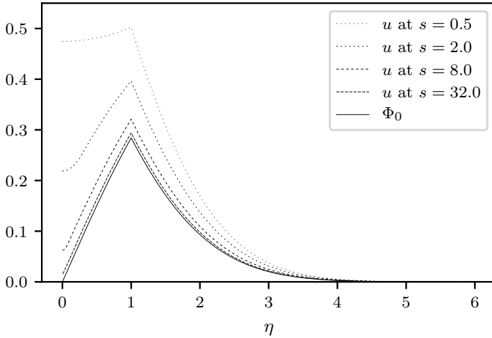
Figure 2. Plot of the function u for \alpha = 1.0 , \beta = 1.0 in the transitional regime with u^* = 0.49 for different times s , together with the conjectured limit profile \Phi_0 .
