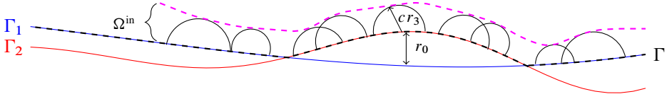
Figure 2. The boundary layer of variable thickness cr_3 .
