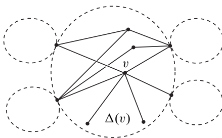
Figure 1. A hub v .
