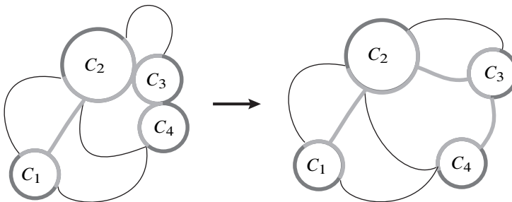
Figure 4. Deforming P_{n,k} to D_{n,k} .
