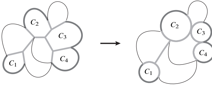
Figure 3. Deforming K_{n,k} to P_{n,k} .
