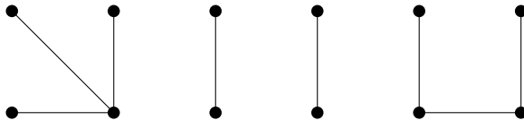
Figure 4. Three subgraphs of K_4 .
