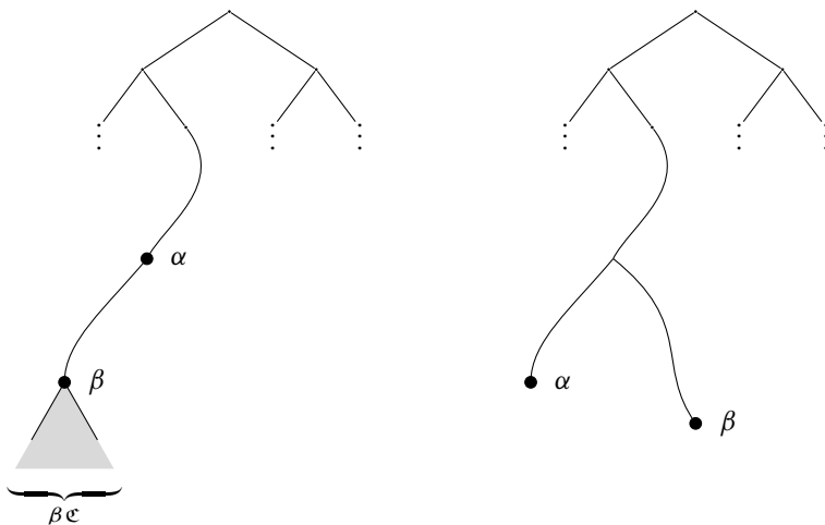
Figure 2. (i) \alpha \preceq \beta (and the paths representing elements of \beta\mathcal{C} ); and (ii) \alpha \perp \beta
