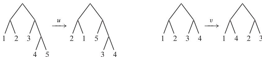
Figure 3. Two elements given by tree-pairs that generate for R. Thompson’s group V
