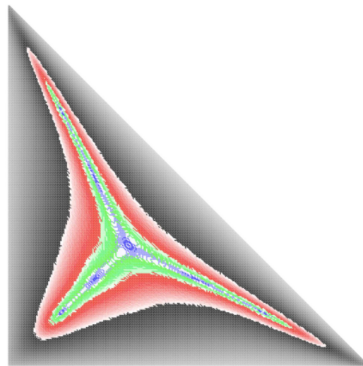
Figure 2. A contour plot for b = 9 with the seven critical points in the Theorem 2.
