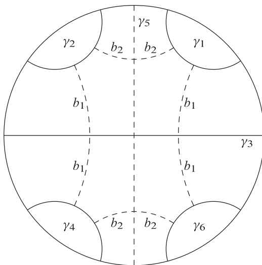
Figure 4. Proof of Lemma 3. Original geodesics \gamma_1, \gamma_2, \gamma_3 and supplementary geodesics \gamma_4, \gamma_5, \gamma_6 .
