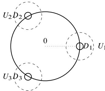
Figure 5. Three circles of reflection on the unit circle and neighbourhoods
