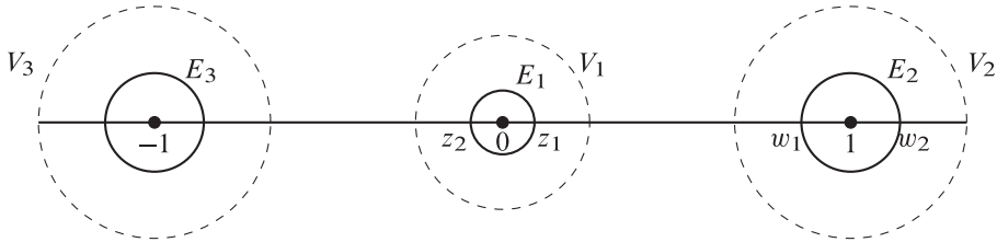
Figure 6. Three circles and their neighbourhoods moved to the real line
