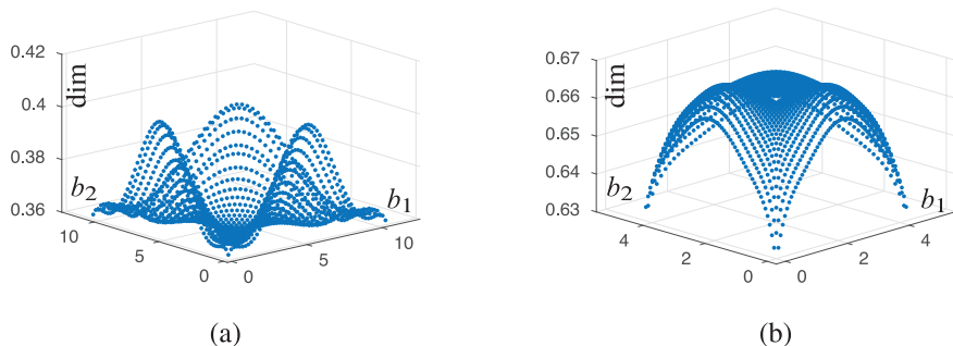
Figure 3. (a) The plot of dimension when b is large ( b = 11 ). (b) The plot of dimension when b is smaller ( b = 4.5 ).
