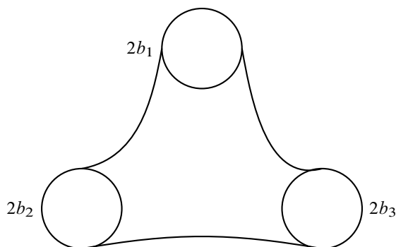
Figure 1. A pair of pants with geodesic boundary curves of lengths 2b_1, 2b_2, 2b_3
