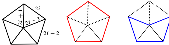
Figure 1. Left: The wheel graph \omega_{2j+1} for j = 2 with edge order indicated. Center: The “exterior” 2j + 1 -gon is the pictured (red) subgraph. Right: The “interior” 2j + 1 -gon is the pictured (blue) subgraph.
