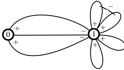
Figure 4. The case j = 3 . The graph \theta_7 (pictured) underlying the element \beta_7 \in \text{B}(\mathcal{H}_{\text{Lie}})(7, 0) . The signs indicate the effect of transposing at the vertices. The bracket labeled by a minus sign indicates that the block permutation exchanging pairs of flags on two loops gives a minus sign. The label of the genus 1 vertex is (up to scalar multiple) the unique class for which \text{Aut}(\theta_7) acts by such signed multiples.
