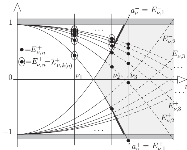
Fig. 1. Depending on the values of \nu , all eigenvalues are achieved by the two families of levels \lambda_{\nu,k}^+ and \lambda_{\nu,k}^- (case \nu = \nu_1 < 2 ), or only some of them (case \nu = \nu_2 \in (2, \sqrt{8}) ). For \nu > \sqrt{8} (case \nu = \nu_3 ), the gap (-1, 1) is contained in (a^+, a^-) and the method does not characterize any eigenvalue in the gap. To clarify the picture, only the family of eigenvalues E_{\nu,n}^+ has been represented, but the family E_{\nu,n}^- is easily recovered by symmetry with respect to the horizontal axis. To take the multiplicity into account, we denote by k(n) the smallest k for which \lambda_{\nu,k}^+ = E_{\nu,n}^+ .
