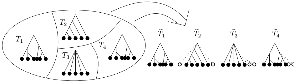
Fig. 2. A schematic description of Ramsey chains and the way they are used to construct approximate distance oracles and approximate ranking data structures. Ramsey chains are obtained by iteratively applying Theorem 3.2 and Lemma 2.1 to find a decreasing chain of subsets X = X_0 \supseteq X_1 \supseteq \dots \supseteq X_s = \emptyset such that X_j can be approximated by a tree metric T_{j+1} . The tree T_{j+1} is, in a sense, a “distance estimator” for X_j \setminus X_{j+1} —it can be used to approximately evaluate the distance from a point in X_j \setminus X_{j+1} to any other point in X_j . These trees form an array which is an approximate distance oracle. In the case of approximate ranking we also need to extend the tree T_{j+1} to a tree on the entire space X using Lemma 4.1. The nodes that were added to these trees are illustrated by empty circles, and the dotted lines are their connections to the original tree.
