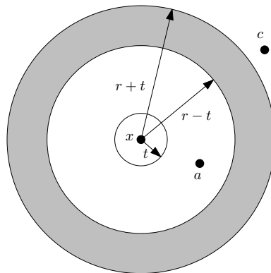
Fig. 1. A schematic description of the lower bound in (3). The clusters that are induced by points which lie outside the ball B_X(x, r+t) , such as c , cannot touch the ball B_X(x, t) . On the other hand, if a point from B_X(x, r-t) , such as a , appeared first in the random order among the points in B_X(x, r+t) then its cluster will “swallow” the ball B_X(x, t) . The probability for this to happen is |B(x, r-t)|/|B(x, r+t)| . Only points in the shaded region can split the ball B_X(x, t) .
