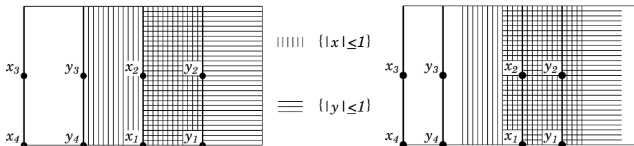
Fig. 4. Examples of the parallelogram [0, \omega_2[ \times [0, \omega_1/\iota[ with its important cycles, on the left for \{N, E, S, W\} and on the right for \{N, E, SE, S, W, NW\} .
