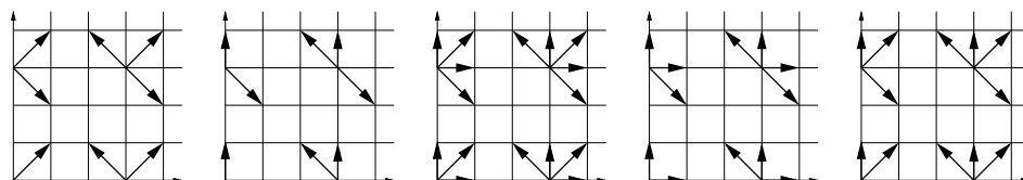
Fig. 2. The five singular walks in the classification of [6].
