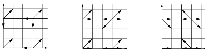
Fig. 1. Three famous examples, known as Kreweras', Gessel's and Gouyou-Beauchamps' walks. They have been, and are still, the object of many studies (see, e.g., [5, 12, 13], [4, 16, 17] and [8, 23], respectively).
