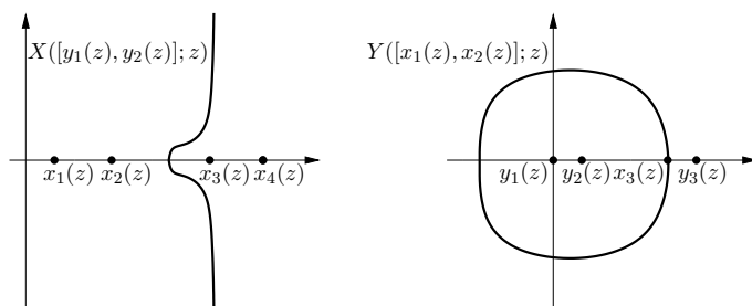
Fig. 3. The curves X([y_1(z), y_2(z)]; z) and Y([x_1(z), x_2(z)]; z) for Gessel's walk.
