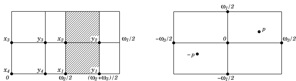
Fig. 5. Domains of definition of \widehat{w} (left) and \bar{w} (right).
