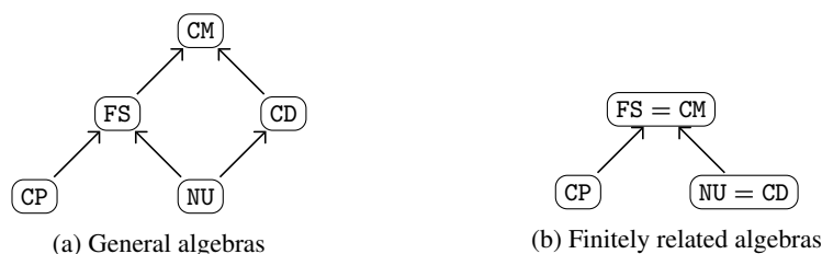
Fig. 1. Comparison of some classes of algebras; arrows depict inclusions.
