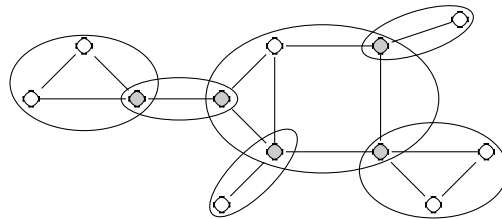
Fig. 2. A graph, its cut vertices (filled-in) and blocks (encircled).
