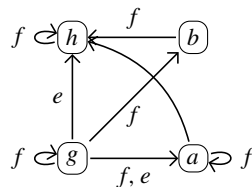
Fig. 8. The final argument for the proof of Lemma 3.8. Label d means that the edge is in Q'(d) .
