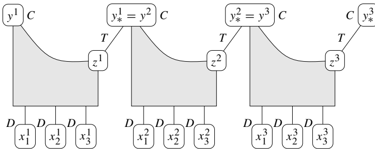
Fig. 4. The second step: formula \Theta for n = l = 3 .
