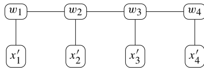
Fig. 5. Graph of a comb-formula for n' = 4 .
