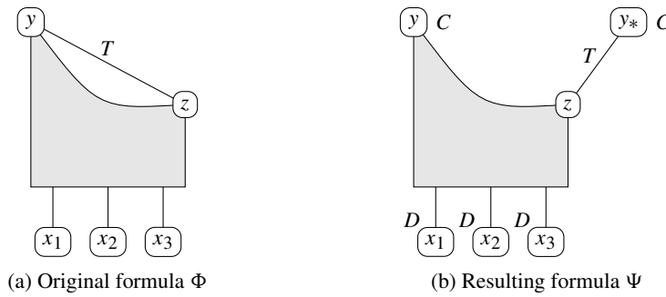
Fig. 3. The first step for n = 3 .
