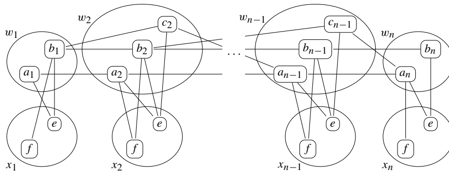
Fig. 7. A comb-formula defining \{e, f\}^n \setminus \{(f, \dots, f)\} .
