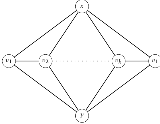
Fig. 3. A double pyramid with apexes x and y .
