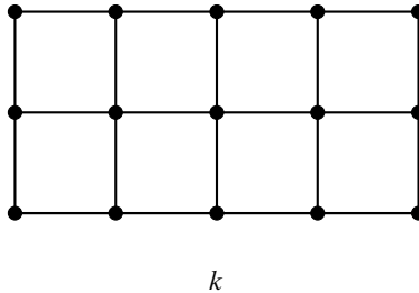
Fig. 4. The double ladder DL_k .
