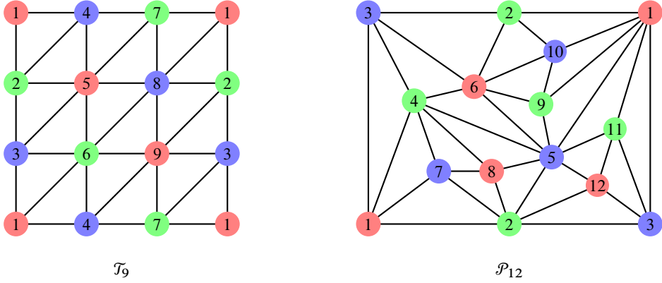
Fig. 2. The edge sets of \mathcal{T}_9 and \mathcal{P}_{12} consist of all the triangles in the respective figures.
