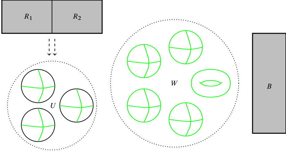
Fig. 6. The situation after finding an almost-spanning collection of spheres; the arrows signify the ability of the spheres in U to absorb any subset of R .
