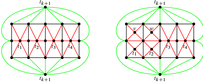
Fig. 5. The absorbing sphere S_U for U is shown on the left; each triangle in the figure corresponds to an edge of \mathcal{H} , which exists because the underlying double ladder lies in L'_U . On the right, we show how S_U can absorb two arbitrary vertices v, w \in U .
