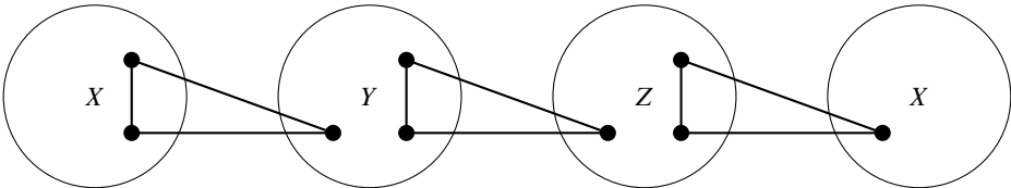
Fig. 1. An extremal construction.
