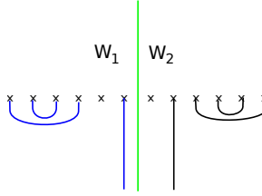
Fig. 11.1. Lagrangian tuples \underline{L}_\lambda (blue, left) and \underline{K}_\mu (black, right).
