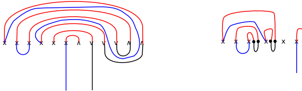
Fig. 12.3. CF(\underline{L}_{\text{hs}}, \widetilde{\underline{L}_{\lambda \sqcup \mu}}) (left) and CF(\underline{L}_{\mu+}, \widetilde{\underline{L}_{\lambda \sqcup \mu-}}) (right).
