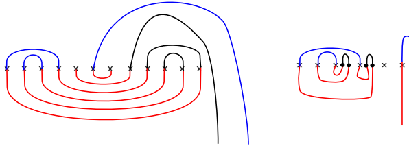
Fig. 12.8. The counterpart of Figure 12.2.
