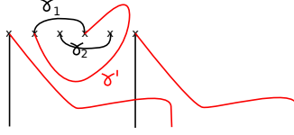
Fig. 5.1. Floer cochain CF(\underline{L}_{\Gamma'}, \underline{L}_{\Gamma}) , where \underline{L}_{\Gamma'} is in red and \underline{L}_{\Gamma} is in black.
