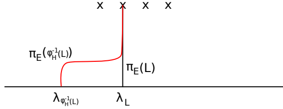
Fig. 2.1. An example of \pi_E(L) (black) and \pi_E(\phi_H^{-1}(L)) (red); crosses are critical values.
