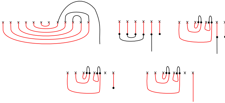
Fig. 12.7. The counterpart of Figure 12.1.
