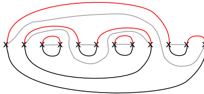
Fig. 6.6. Here \bar{\lambda} is red, \tilde{\lambda}' is grey, and \underline{\lambda}' is black.
