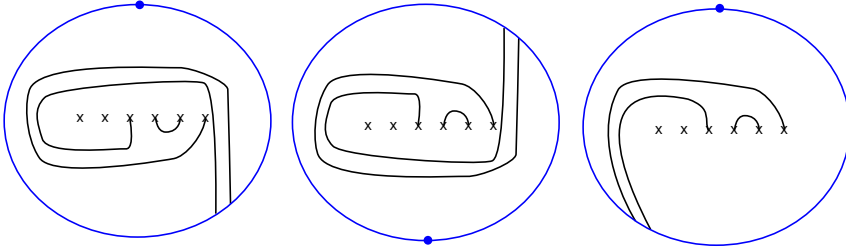
Fig. 10.1. An example of \tau^{-1}(\underline{L}_{\underline{\lambda}}) (left), \iota_E \circ \tau^{-1}(\underline{L}_{\underline{\lambda}}) (middle) and \Psi \circ \iota_E \circ \tau^{-1}(\underline{L}_{\underline{\lambda}}) (right).
