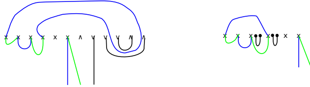
Fig. 12.4. CF(\underline{L}_{\lambda_0 \sqcup \mu}, \underline{L}_{\lambda_1 \sqcup \mu}) (left) and CF(\underline{L}_{\lambda_0 \sqcup \mu^-}, \underline{L}_{\lambda_1 \sqcup \mu^-}) (right).
