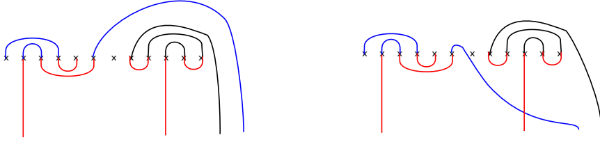
Fig. 12.10. Floer cochain CF(\underline{L}_{\bar{\lambda}}^! \sqcup \underline{K}_{\bar{\mu}}^!, \underline{L}_{\bar{\lambda}'} \sqcup \underline{K}_{\bar{\mu}'}) (left) and CF(\underline{L}_{\bar{\lambda}} \sqcup \underline{K}_{\bar{\mu}}, \underline{L}_{\bar{\lambda}'} \sqcup \underline{K}_{\bar{\mu}'}) (right). The intersection between the positive wrapping of \underline{L}_{\bar{\lambda}} and \underline{K}_{\bar{\mu}} cannot contribute a generator to CF(\underline{L}_{\bar{\lambda}} \sqcup \underline{K}_{\bar{\mu}}, \underline{L}_{\bar{\lambda}'} \sqcup \underline{K}_{\bar{\mu}'}) so the Floer cochain splits.
