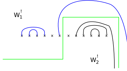
Fig. 11.2. Lagrangian tuples \underline{L}_{\lambda}^! (blue) and \underline{K}_{\mu}^! (black).
