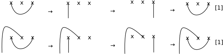
Fig. 3.1. The top row represents an exact triangle in \mathcal{FS}(\pi_E) when E is the A_2 Milnor fibre. The bottom row is exact in \mathcal{FS}^{\text{cyl},2}(\pi_E) by Corollary 3.5.
