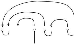
Fig. 9.4. The weight and the cap diagram on top are \lambda_0 and \bar{\lambda_0} ; the weight and the cup diagram on the bottom are \lambda_1 and \underline{\lambda_1} .
