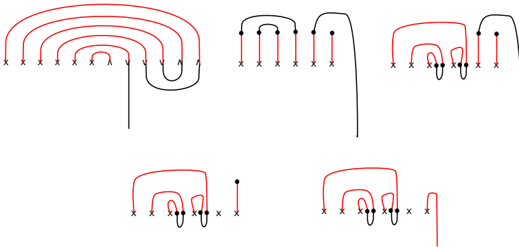
Fig. 12.1. Turning \underline{L}_{\text{hs}} (red) and \underline{K}_\mu (black) to \underline{L}_{\mu^+} (red) and \underline{L}_{\mu^-} (black), respectively.
