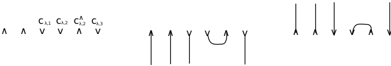
Fig. 6.7. From left to right: a weight \lambda , the cup diagram \underline{\lambda}^{\text{alg}} and the cap diagram \bar{\lambda}^{\text{alg}} .
