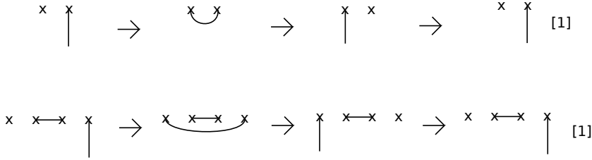
Fig. 9.5. The first row represents an exact triangle in the induction hypothesis. The second row is the exact triangle after applying the ‘cup functor’ \cup_{2,3} to it.
