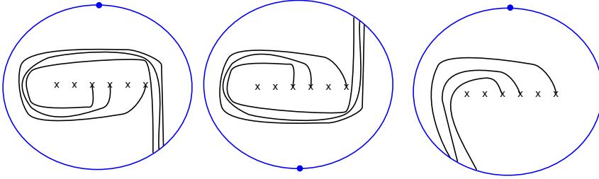
Fig. 10.2. An example of \tau^{-1}(\underline{T}^{\lambda^{-1}(\vee)}) (left), \iota_E \circ \tau^{-1}(\underline{T}^{\lambda^{-1}(\vee)}) (middle) and \Psi \circ \iota_E \circ \tau^{-1}(\underline{T}^{\lambda^{-1}(\vee)}) (right).
