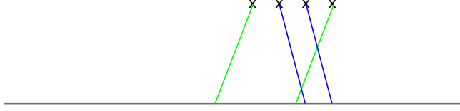
Fig. 4.2. \text{Sym}(\underline{T}_1^{I_0}) \cap \text{Sym}(\underline{T}_1^{I_1}) = \emptyset .
