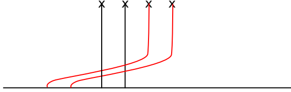
Fig. 2.2. Lagrangian tuples \pi_E(\underline{L}_0) (black) and \pi_E(\phi_{H'_{\underline{L}_0, \underline{L}_1}}^{-1}(\underline{L}_1)) (red) for H'_{\underline{L}_0, \underline{L}_1} \in H_\gamma(E) .
