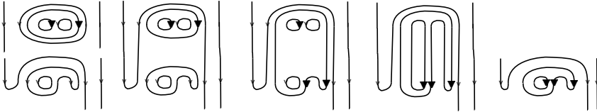
Fig. 9.1. From left to right: y (top) and x_{\min} (bottom) before taking product; successively applying two TQFT operations to the first picture; the product x . Clockwise orientations on circles are indicated by ▼. We choose \gamma_j to be the outermost upper arcs in the 2-circle components of x ; this forces the indicated ▼s on y .
