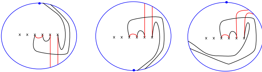
Fig. 9.6. CF(\underline{L}_\lambda, \underline{L}_{\lambda'}) (left), CF(\iota_E(\underline{L}_{\lambda'}), \iota_E(\underline{L}_\lambda)) in \mathcal{F} \mathcal{S}^{\text{cyl},n}(\pi_E)^\dagger (middle) and CF(\Psi \circ \iota_E(\underline{L}_{\lambda'}), \Psi \circ \iota_E(\underline{L}_\lambda)) (right). The dot on the boundary indicates the stop.
