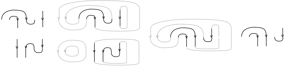
Fig. 9.3. From left to right: 1) two oriented circle diagrams \underline{\lambda}\lambda a , b\lambda\bar{\lambda} , 2) closure of the oriented circle diagrams, all circles are oriented counterclockwise (see Section 6.4), 3) taking product, 4) removing the completion (grey).
