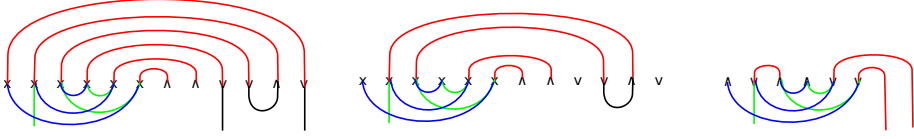
Fig. 12.2. CF(\underline{L}_{\text{hs}}, \iota_j(\underline{L}_\lambda, \underline{K}_\mu)) (left) and CF(\underline{L}_{\mu+}, \underline{L}_{\lambda \sqcup \mu-}) (right).
