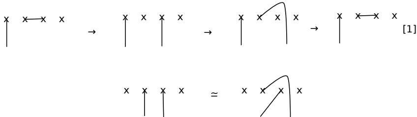
Fig. 5.4. The top row is an exact triangle so the third term is generated by the first and second terms, which are in turn generated by \{\underline{T}^I\}_{I \in \mathcal{J}} . The second row represents two quasi-isomorphic objects.
