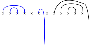
Fig. 12.9. Lagrangian tuples \underline{L}_{\bar{\lambda}} (blue) and \underline{K}_{\bar{\mu}} (black).
