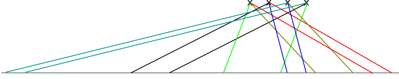
Fig. 4.1. The case when s = 4 and n = 2 .
