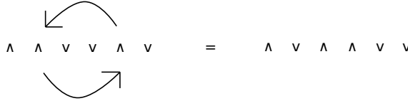
Fig. 9.7. Left: a weight \lambda . Right: the weight PD(\lambda) .
