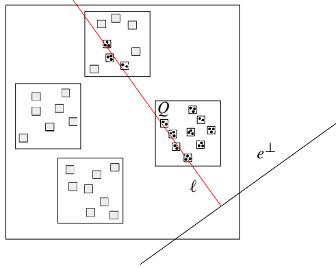
Fig. 1. The red line \ell is in \mathcal{L}_b : it hits many cubes in \mathcal{Q}_\delta(Q) but not K \cap Q .
