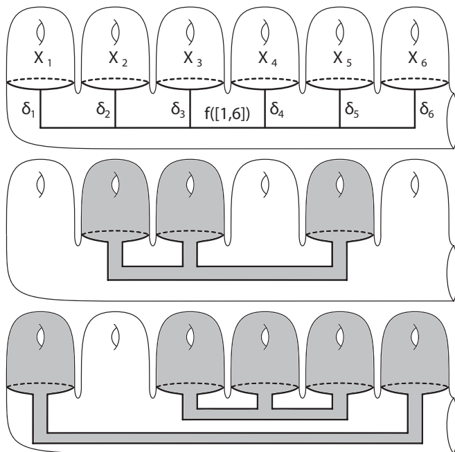
Fig. 2. On the top are the X_i and the \delta_i and f([1, g]) for g = 6 . In the middle is \Sigma_{\{2,3,5\}} , and on the bottom is \Sigma_{\{3,4,5\}} isotoped to be disjoint from \Sigma_{\{1,6\}} .
