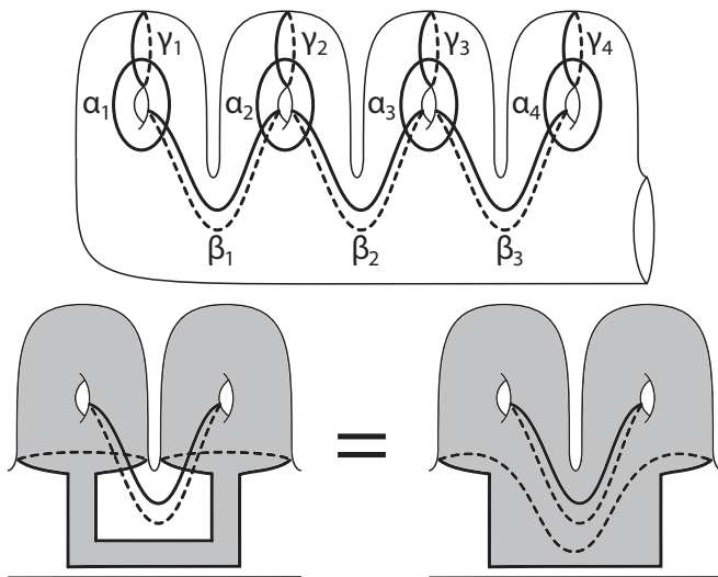
Fig. 3. On the top are the generators for \Gamma = \text{Mod}_g^1 , drawn in such a way that it is clear how they interact with the subsurfaces \Sigma_I . On the bottom we illustrate why \beta_j lies in a surface isotopic to \Sigma_{j,j+1} , and thus why the Dehn twist T_{\beta_j} lies in \Gamma_{j,j+1} .
