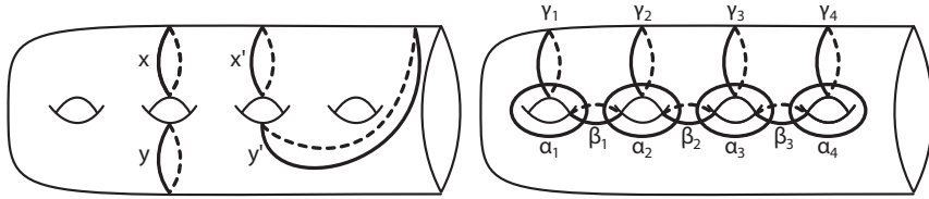
Fig. 1. On the left are two genus-1 BP maps \varphi = T_x T_y^{-1} and \psi = T_{x'} T_{y'}^{-1} that are adjacent in \text{BP}(\mathcal{J}_g^1) . On the right are the Dehn twists involved in the definition of the set S . Note that x' and y' on the left are disjoint from \alpha_2 , so \psi = T_{x'} T_{y'}^{-1} commutes with T_{\alpha_2} .
