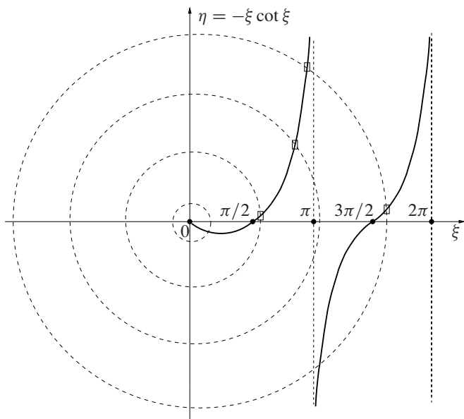
Figure 4. Graphical solution of system (2.12).
