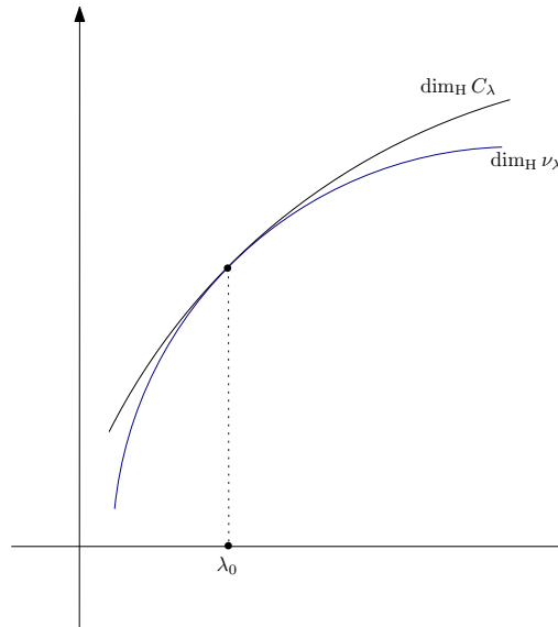
Figure 2. Graphs of \dim_H C_\lambda and \dim_H \nu_\lambda as functions of \lambda .
