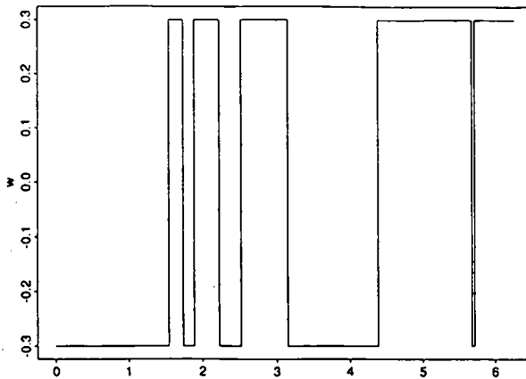
Figure 3: The suboptimal control function w
