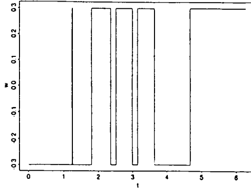
Figure 1: The suboptimal control function w
