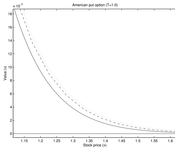
FIG. 4. “Zoom-in plots” of the exact solution (solid line), the predictor-corrector solution (dashed line), and the penalty solution (dotted line).
