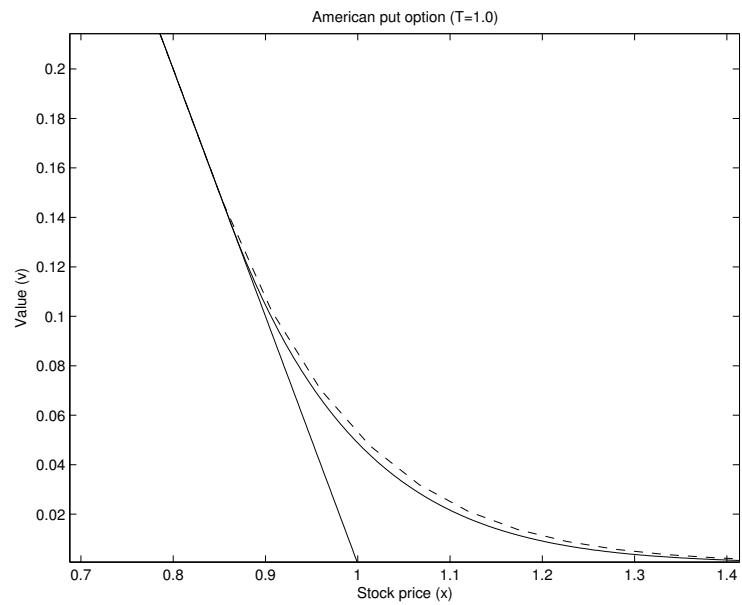
FIG. 2. The price of the American put option with expiration time T = 1.0 : the exact solution along with the payoff function (solid line) and the Brennan and Schwartz solution (dashed line)
