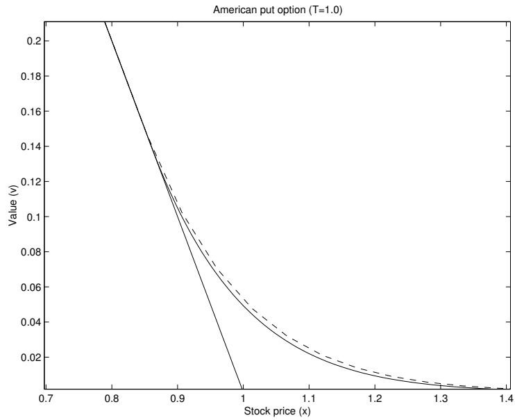
FIG. 1. The price of the American put option with expiration time T = 1.0 : the exact solution along with the payoff function (solid line) and the predictor–corrector solution (dashed line)
