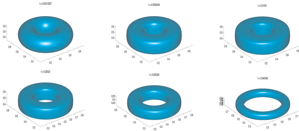
FIG. 6. \phi_4^0(\xi) -evolution from an initial torus, at different times
