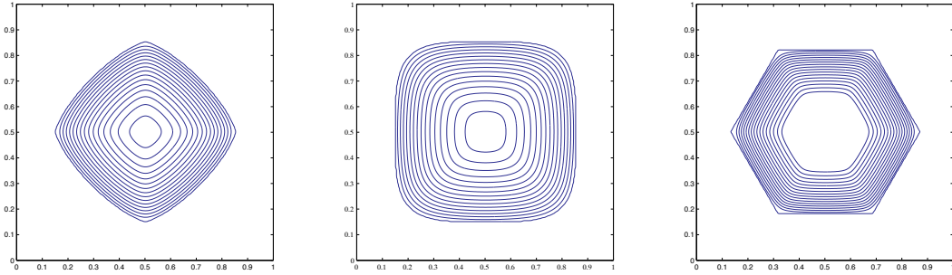
FIG. 3. \Omega(t) at different times for the anisotropic densities \phi_1, \phi_2, \phi_3
