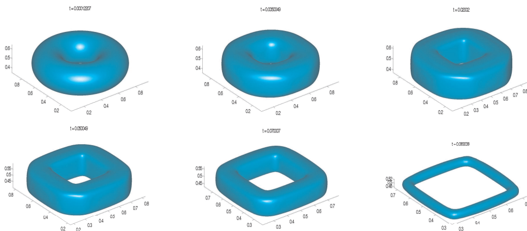
FIG. 7. \phi_5^0(\xi) -evolution from an initial torus, at different times
