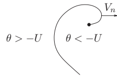
FIG. 1. Motion of the spiral. Here \theta is the angle in polar coordinates.
