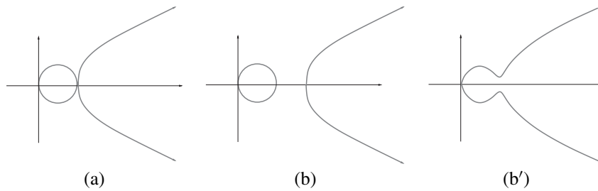
FIG. 3. Different evolutions for non spiral initial data
