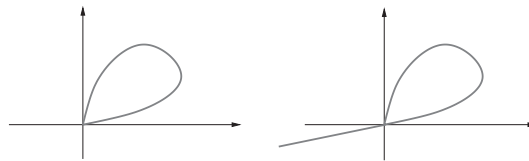
FIG. 2. Examples of non spiral initial data
