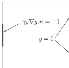
FIG. 3. Boundary conditions for the V-shaped conductor. An homogeneous Neumann condition is prescribed on the non-specified boundaries.
