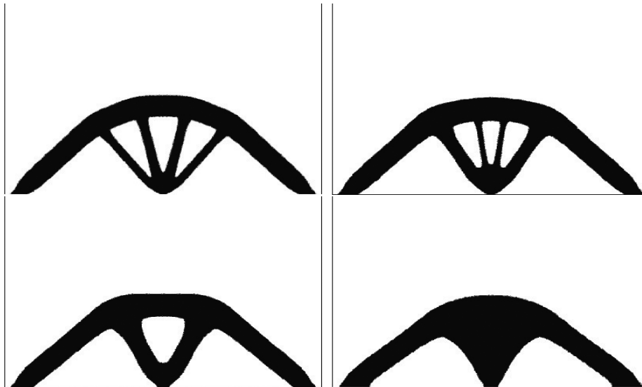
FIG. 9. Bridge for \alpha = 0.2, 1, 3, 10 , respectively
