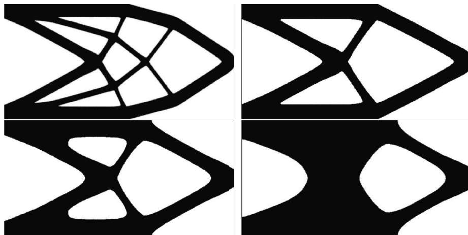
FIG. 8. Cantilever for \alpha = 0.1, 2, 20, 50 , respectively
