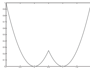
FIG. 1. Plot of the function \mathcal{W}
