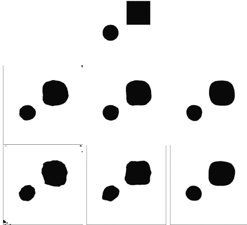
FIG.2. Source identification. Top: True sources. Then reconstructed sources for R = 33\% (first line) and R = 58\% (second line) with \alpha = 10^{-8} (first column), \alpha = 10^{-7} (second column) and \alpha = 10^{-6} (third column).
