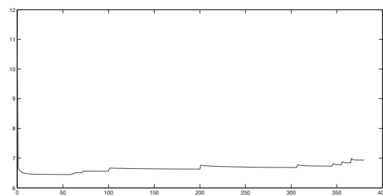
FIG. 7. Convergence history for the optimal heater problem ( \alpha = 0.1 ), with the number of iterations on the x-axis and the values of the criterion on the y-axis.
