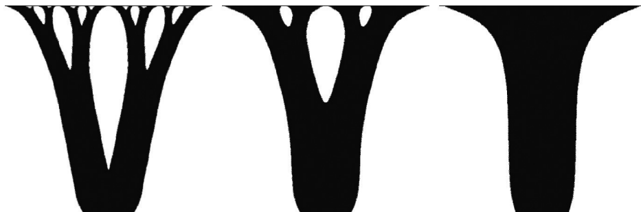
FIG. 6. Optimized heater for \alpha = 0.1, 0.5, 2 , respectively
