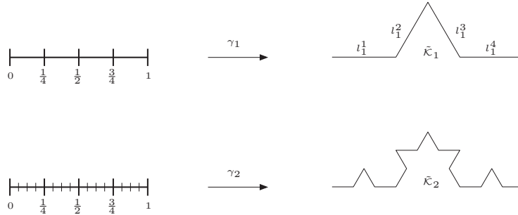
FIG. 1. The first and second iterations in the construction of the natural parametrization \gamma of the von Koch curve
