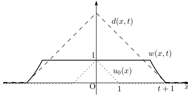
FIG. 2. The graph of w when t \geq \log 2
