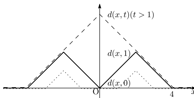
FIG. 1. The graph of d
