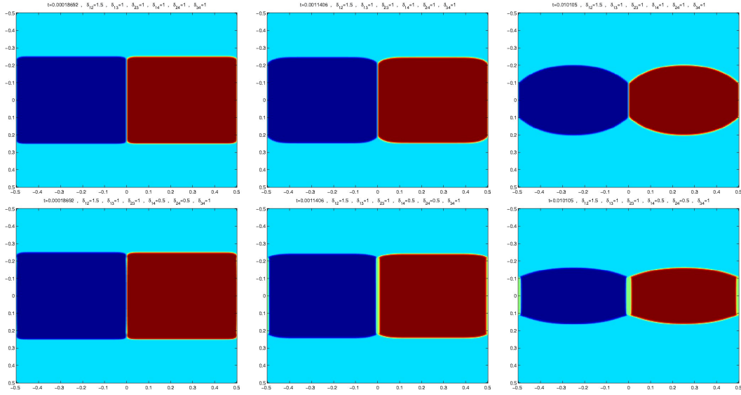
FIG. 6. Starting from 3 phases out of 4, a nucleation may occur when the triangle inequality is not satisfied. First line: \sigma_{1,2} = 1.5, \sigma_{1,3} = 1, \sigma_{2,3} = 1, \sigma_{1,4} = 1, \sigma_{2,4} = 1, \sigma_{3,4} = 1 (no nucleation, triangle inequality holds); Second line with \sigma_{1,2} = 1.5, \sigma_{1,3} = 1, \sigma_{2,3} = 1, \sigma_{1,4} = 0.5, \sigma_{2,4} = 0.5, \sigma_{3,4} = 1 (nucleation occurs, \sigma_{1,2} > \sigma_{1,4} + \sigma_{2,4} ). [Colors shown in the online version]
