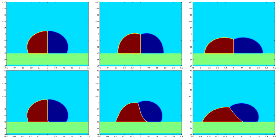
FIG. 9. Dynamics of two droplets. First line: \sigma_{i,j} = 1 ; second line: \sigma_{1,2} = 1, \sigma_{1,3} = 1, \sigma_{2,3} = 0.9, \sigma_{1,4} = 1, \sigma_{2,4} = 0.7 , and \sigma_{3,4} = 1.3 . [Colors shown in the online version]
