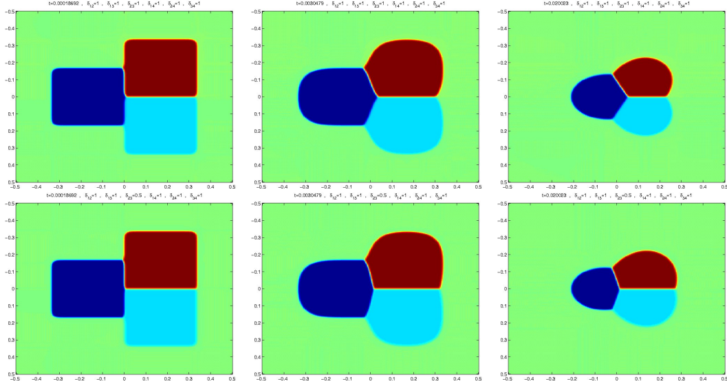
FIG. 5. Evolution of a 4-partition; first line: \sigma_{i,j} = 1 ; second line: \sigma_{1,2} = 1, \sigma_{1,3} = 1, \sigma_{2,3} = 0.5, \sigma_{1,4} = 1, \sigma_{2,4} = 1, \sigma_{3,4} = 1 . [Colors shown in the online version]
