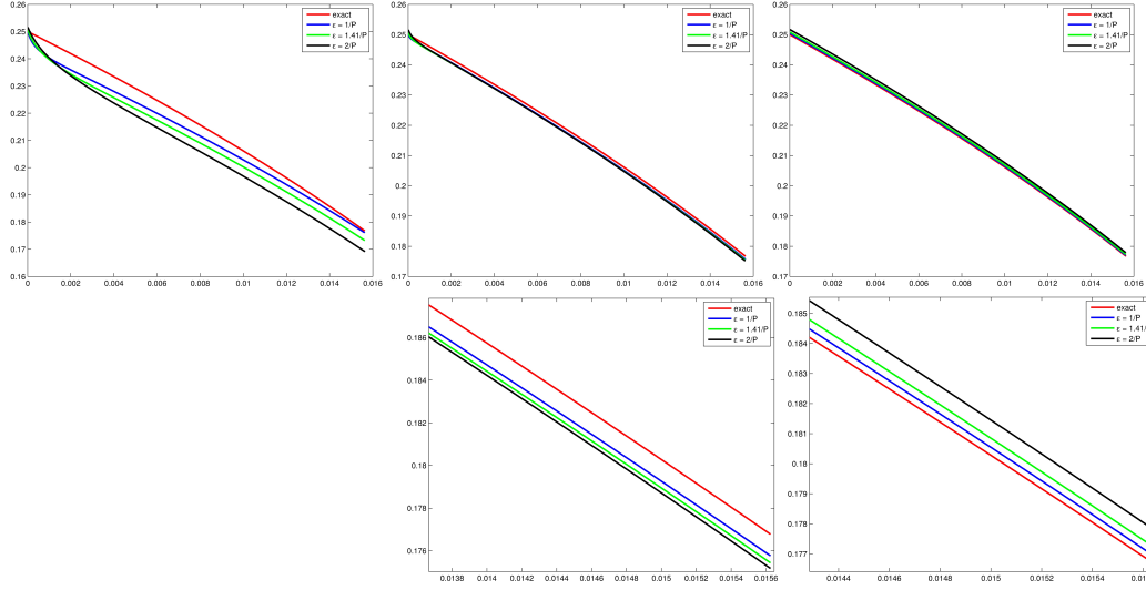
FIG. 4. The graphs of t \rightarrow R_\epsilon(t) for \epsilon = 1/P , \epsilon = \sqrt{2}/P and \epsilon = 2/P , compared with the exact solution. Left to right: with potentials \mathbf{W}_1 , \mathbf{W}_2 , and \mathbf{W}_\sigma . Second line: Zoom on the first line. [Colors shown in the online version]
