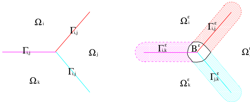
FIG. 1. \epsilon -partition of \Omega [Colors shown in the online version]
