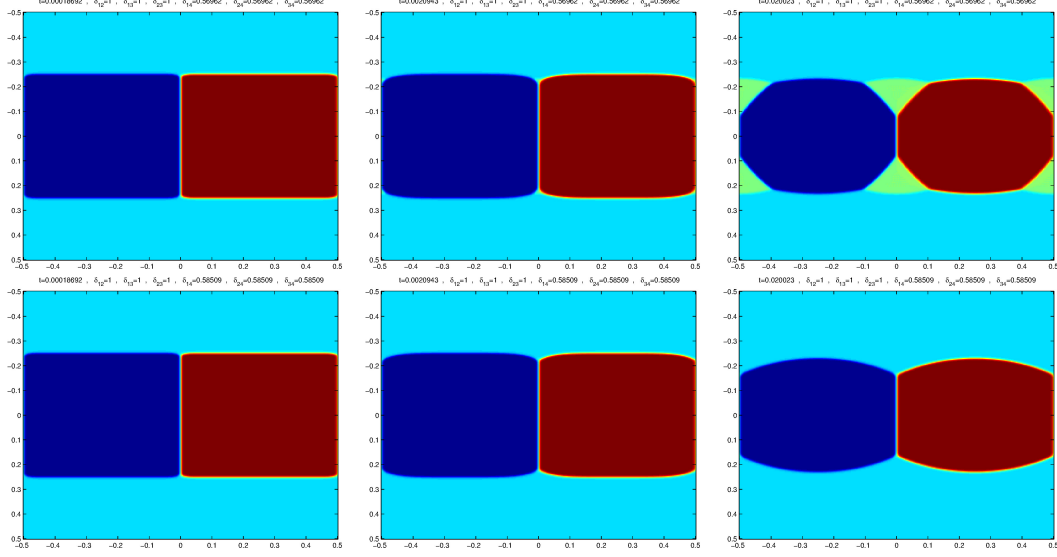
FIG. 7. A nucleation example in the case \sigma_{1,2} = 1 , \sigma_{1,3} = 1 , \sigma_{2,3} = 1 , \sigma_{1,4} = 1/2 + \varepsilon , \sigma_{2,4} = 1/2 + \varepsilon , \sigma_{3,4} = 1/2 + \varepsilon . First line with \varepsilon = \frac{0.9(2-\sqrt{3})}{2\sqrt{3}} (triple points are unstable, the triangle inequality holds but the configuration with a triple point between phases 1,2,3 has larger energy than a triangle containing only phase 4; second line with \varepsilon = \frac{1.1(2-\sqrt{3})}{2\sqrt{3}} (triple points are stable). [Colors shown in the online version]
