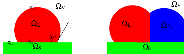
FIG. 2. Wetting of droplets on a solid surface. The contact angle \theta satisfies Young's law. [Colors shown in the online version]
