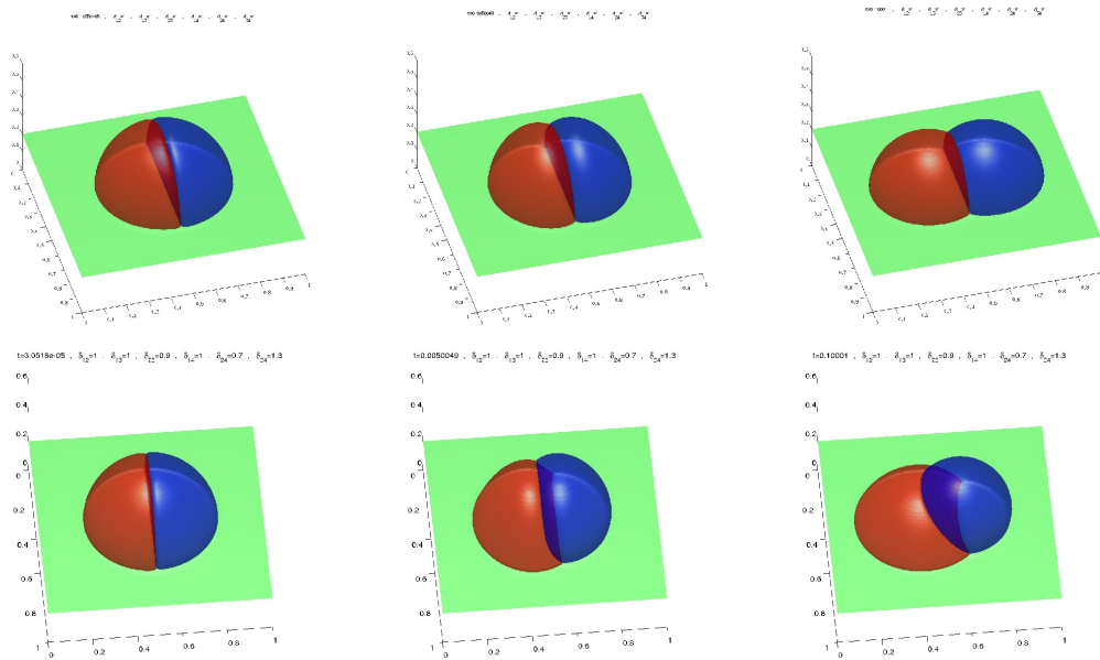
FIG. 10. Dynamics of two droplets in 3D. First line: \sigma_{i,j} = 1 ; Second line: \sigma_{1,2} = 1, \sigma_{1,3} = 1, \sigma_{2,3} = 0.9, \sigma_{1,4} = 1, \sigma_{2,4} = 0.7 , and \sigma_{3,4} = 1.3 . [Colors shown in the online version]
