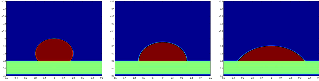
FIG. 8. Optimal shape of a droplet. Left: \sigma_{1,2} = 1, \sigma_{1,3} = 0.5, \sigma_{2,3} = 1 ; middle: \sigma_{1,2} = 1, \sigma_{1,3} = 1, \sigma_{2,3} = 1 ; right: \sigma_{1,2} = 1, \sigma_{1,3} = 1, \sigma_{2,3} = 0.5 . [Colors shown in the online version]
