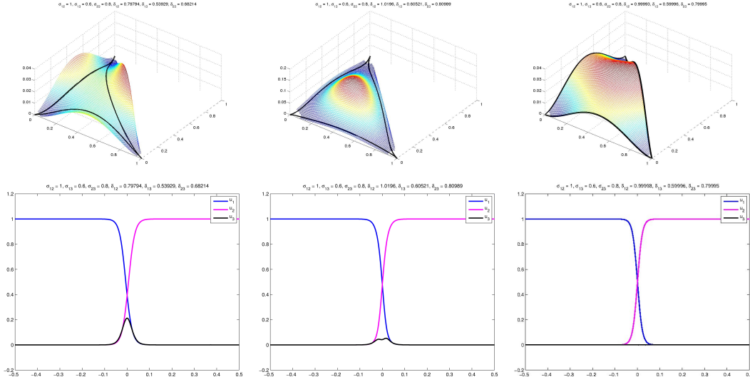
FIG. 3. First line: Geodesics p_{ij} between phases e_i and e_j , i, j \in \{1, 2, 3\} , Second line: values of u_1 , u_2 , u_3 along geodesic p_{12} (from left to right: with potentials W_1 , W_2 and W_\sigma ) [Colors shown in the online version]
