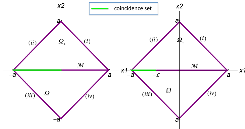
FIG. 3. Domains \Omega_+ and \Omega_- ; coincidence sets for u and v_1 (left) and for v_{3,\varepsilon} (right)
