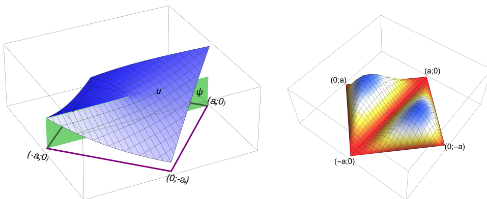
FIG. 4. The exact solution u (left) and the function v_1 - u (right)
