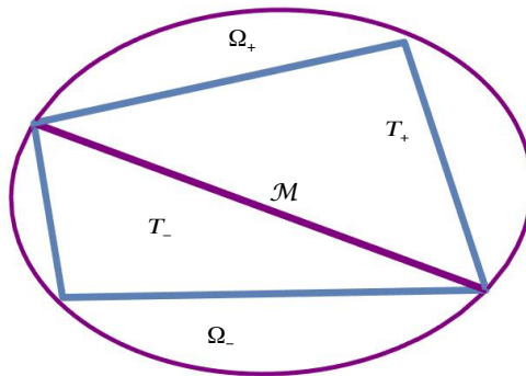
FIG. 2. Triangles T_+ and T_-
