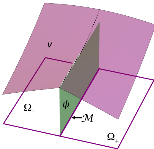
FIG. 1. The thin obstacle problem
