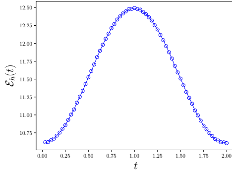
Figure 7. Energy \mathcal{E}_h(t) for experiment in Section 4.1.4.
