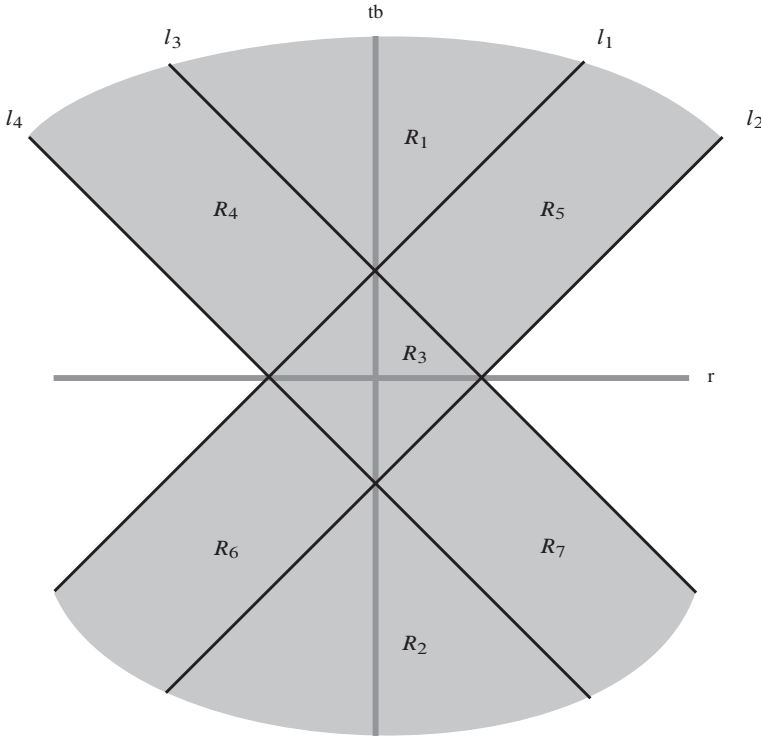
Figure 2. A non-loose knot must map to the grey region under the map \Phi . The black lines, labeled l_1, \dots, l_4 , break the grey region into seven subregions as indicated in the figure. The regions R_i are open regions (that is not including the points on the black lines).
