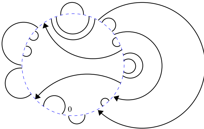
(c) Type- \gamma configuration.
