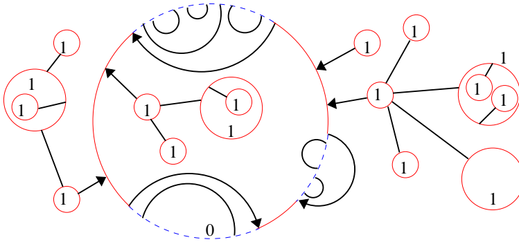
(e) Type- \epsilon configuration.
