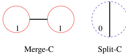
Figure 2.5. The labeled configurations that contribute to the function \mathfrak{b} .
