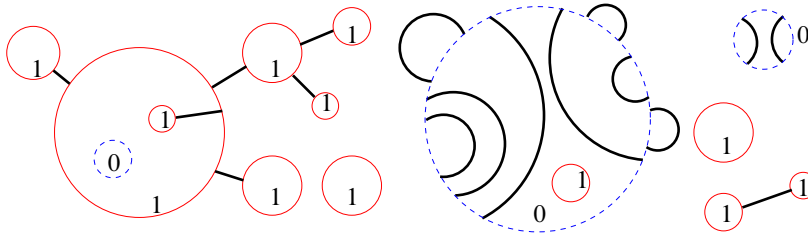
Figure 3.1. A labeled configuration that contributes to \mathfrak{h} .
