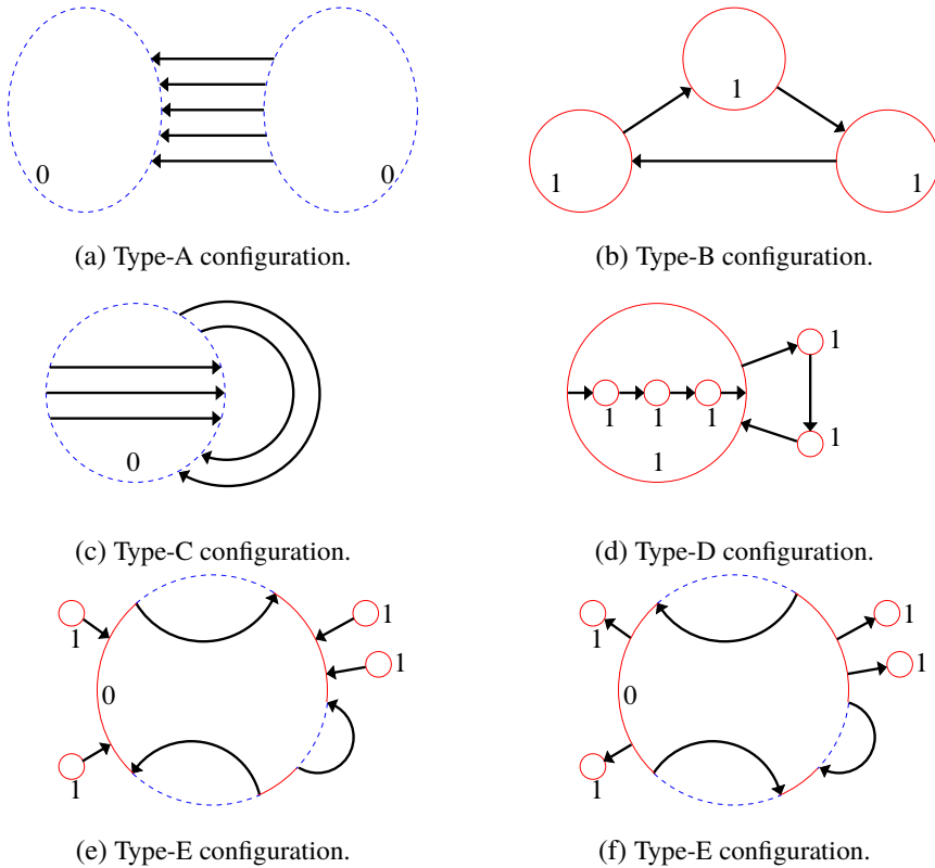
Figure 2.6. The oriented labeled configurations that contribute to the function \partial .
