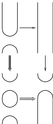
Figure 4.2. The partial cube of resolutions of D' for the RII invariance. We cancel along the double arrows leaving a subquotient complex isomorphic to the complex for D .
