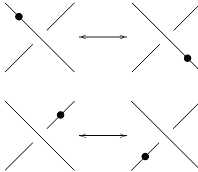
Figure 4.4. Additional moves for the basepoint.
