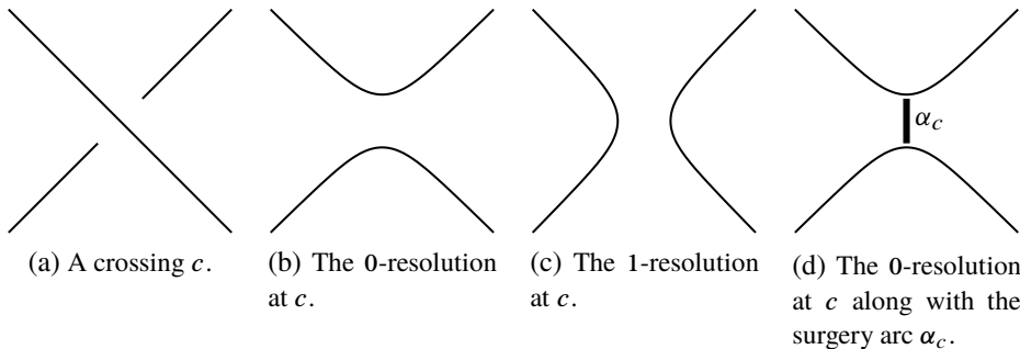
Figure 2.1. A crossing, its 0-resolution, its 1-resolution, and its 0-resolution along with the surgery arc. If we forget the surgery arc, we get the 0-resolution; and if we perform embedded surgery along it, we get the 1-resolution.
