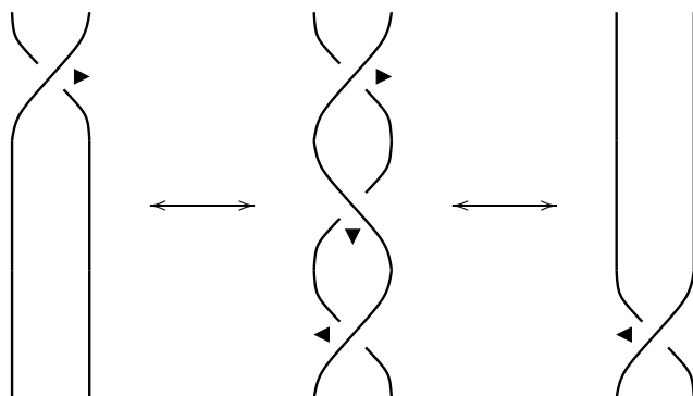
Figure 4.5. Changing the decoration at a single crossing.
