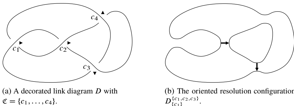
Figure 2.3. A decorated link diagram for the figure eight knot, and one of the induced oriented resolution configurations.
