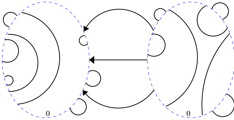
(a) Type- \alpha configuration.
