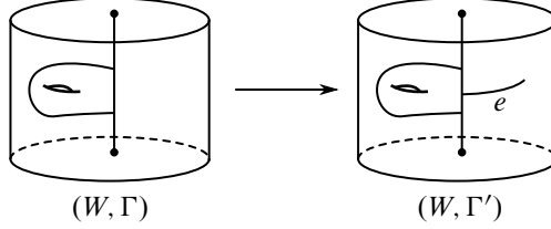
Figure 5.1. Adding an interior leaf to a graph cobordism.
