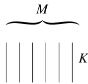
Figure 2. A fibration.
