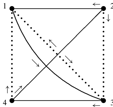
Figure 4. An automaton.
