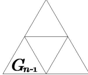
Figure 8. G_n (if f(n) = 0 )
