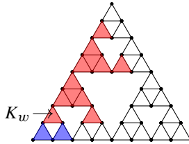
Figure 3. The set U is drawn in red. The two blue cells correspond to K_w^* .
