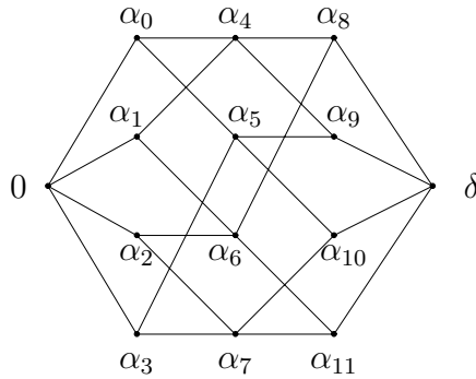
FIGURE 4: The digraph G_0 corresponding to the Kac-Moody algebra \mathfrak{g}(A_3^{(1)}) .
