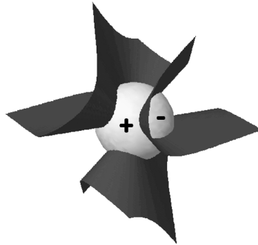
Figure 1: The variety h^{-1}(0) separates the sphere S^2 into 2 components.
