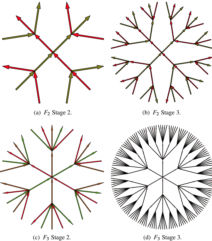
Figure 2. Cayley graphs for F_2 and F_3 .
