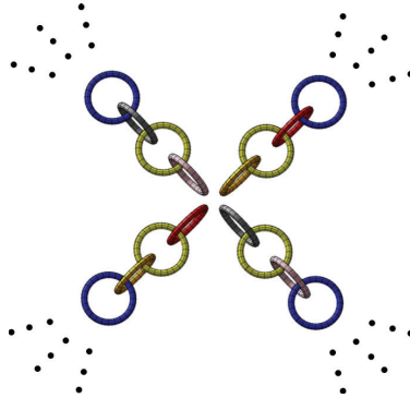
Figure 6. Start of construction for \mathcal{C}_1 and \mathcal{C}_2 in the case F(2).
