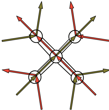
Figure 4. Balls, tubes around G(F_2) .
