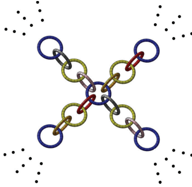
Figure 5. Construction of rigid Cantor sets placement for G(F_2) .
