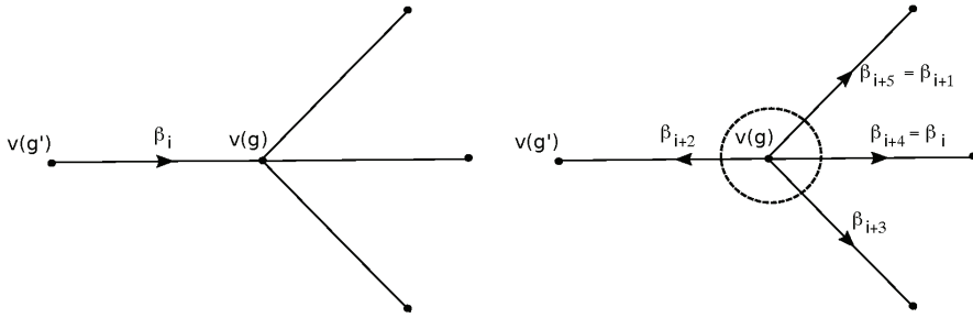
Figure 3. Inductively labelling edges.
