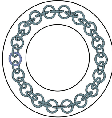
Figure 1. Two stages for an Antoine construction.
