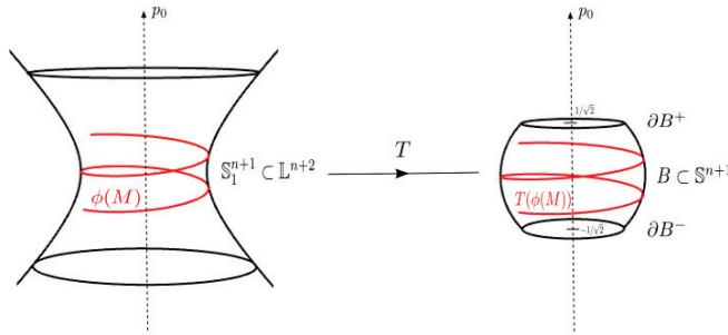
Figure 1. Lorentz–Minkowski space \mathbb{L}^{n+2} and Klein model of \mathbb{S}_1^{n+1} .
