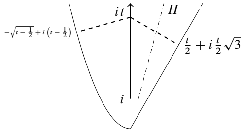
Figure 2. The domain \Xi(2, \pi/6) .
