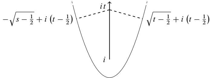
Figure 1. The domain \Pi_\alpha with \alpha = 2 .
