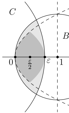
Figure 4. The lower bound for \mathcal{L}(B \cap C) in the proof of Lemma 5.5.
