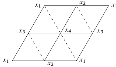
Figure 2. Degree-two ramified cover of the tetrahedral sphere.
