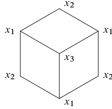
Figure 1. Degree-three ramified cover of the Calabi–Croke sphere.
